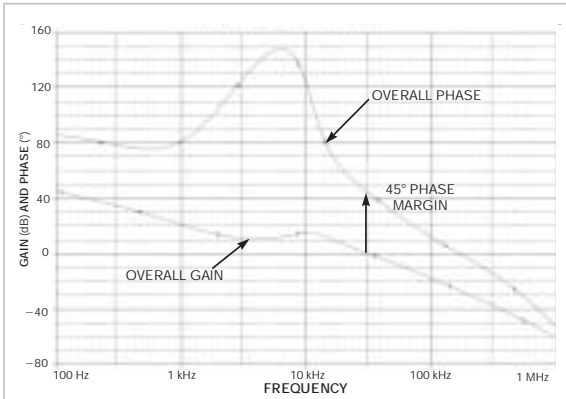
Figure 5 The phase-angle plot for the circuit of Figure 4 shows a sufficient phase-angle margin to allow stable operation with a ceramic output-filter capacitor.
