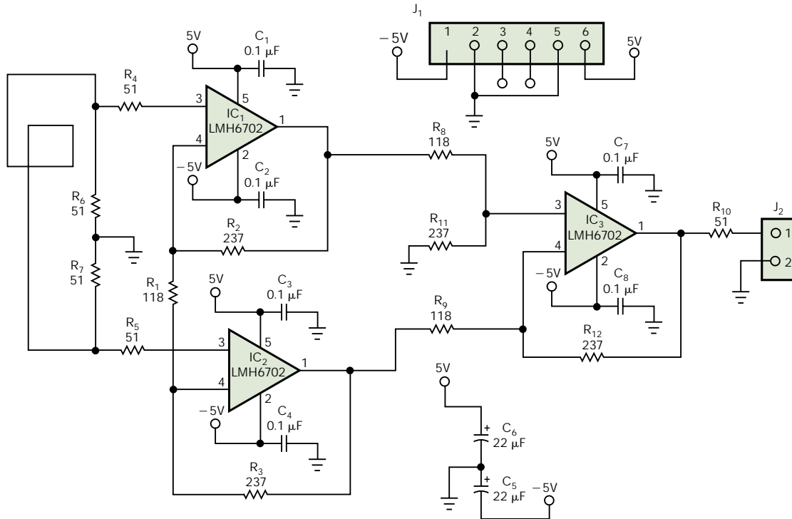
Figure A This high-bandwidth, 20-dB preamplifier amplifies the small signals that the magnetic loop picks up.
