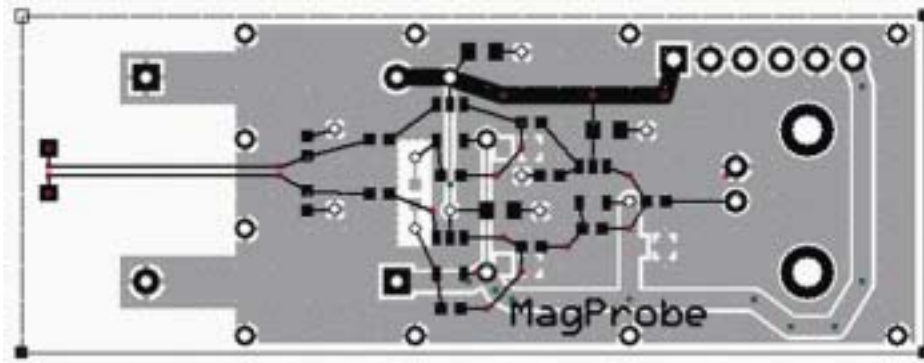
Figure B The amplifier layout is orthogonal to the probe tip and as balanced as possible.
