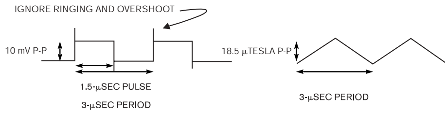
Figure A This typical time-domain measurement converted to the B-field is a 3-μsec, 50%-duty-cycle switching waveform. The 5-mV peak measurement equates to a 12.3-tesla/sec rate of change in flux density.
