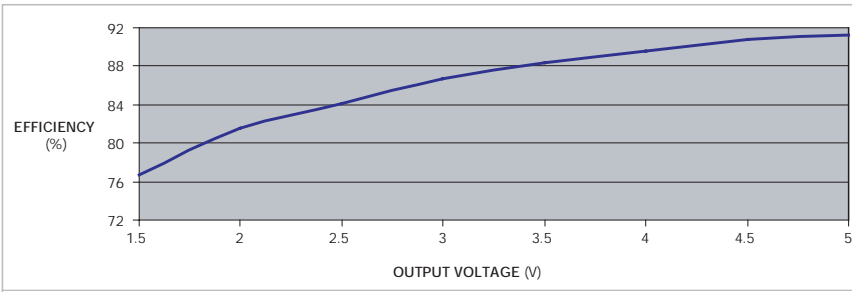
Figure 2 The regulator cascade's combined efficiency improves as the unregulated output voltage increases.
