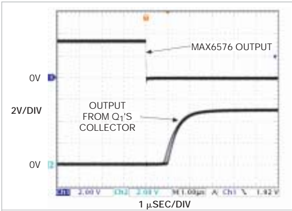
Figure 3 As in Figure 2, Q 1 's average output jitter with respect to IC 1 's negative-going output also averages less than 1 μsec.
