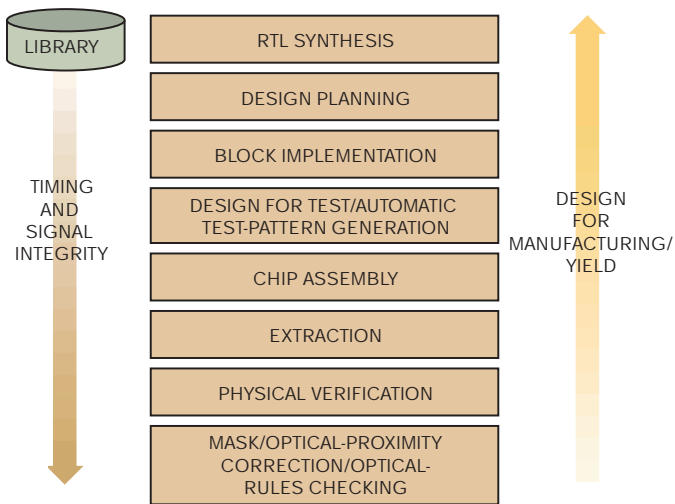
Figure 3 The CIS Alliance selected a DFM flow.
