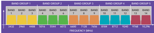
Figure B The WiMedia ultrawideband radio employs 14 channels and uses frequency hopping to mitigate interference.
