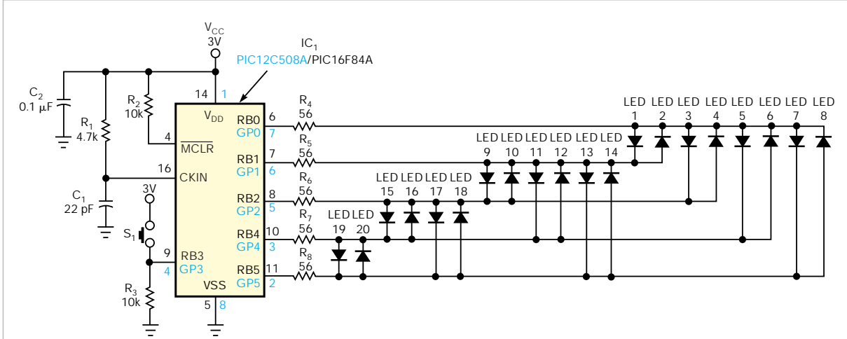
Figure 1 A dot- or bar-graph display uses either a one-time-programmable PIC12C508A or, for experimentation, a reprogrammable and reusable PIC16F84A. Use high-brightness diodes for LED 1 through LED 20.
