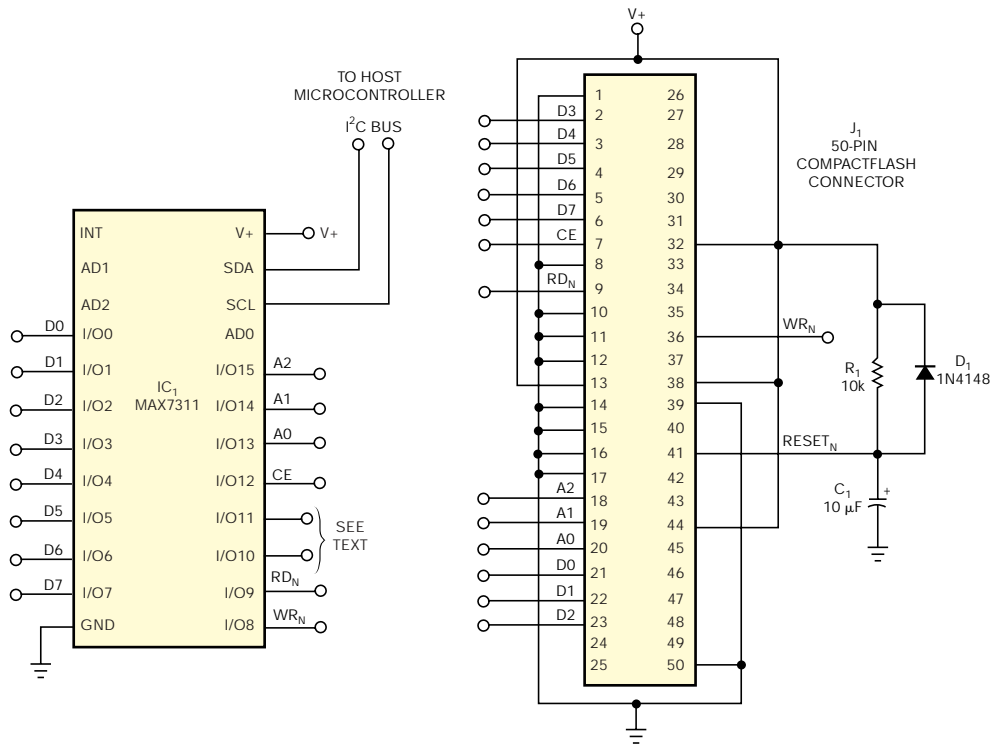
Figure 1 A 16-bit I/O extender, IC 1 , and a CompactFlash connector add external data storage to a microcontroller's I 2 C bus.
