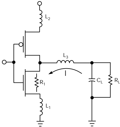
Figure 1 L_1 , L_2 , and L_3 represent the bond wires inside an IC. Fast-changing currents in these wires create appreciable voltages in these wires (courtesy Fairchild Semiconductor).
