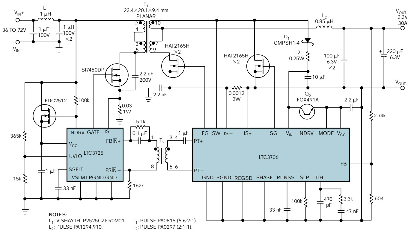
Figure 3 The LTC3706 secondary-side synchronous controller and its companion smart gate driver, the LTC3725, make it possible to create an isolated forward converter with the simplicity and performance of a buck regulator.
