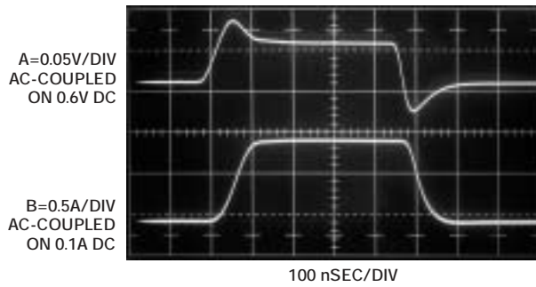
Figure 10 Figure 8's bipolar-output-load-tester response is two times slower than the FET version, but the circuit is simpler and eliminates compensation trims. Trace A is A_1 's output, and Trace B is Q_1 's collector current.
