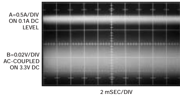
Figure 14 This waveform has the same conditions as Figure 13, except with increased noise bandwidth of 5 MHz, exceeding the regulator's bandwidth and resulting in 50-mV-p-p output error.
