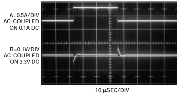
Figure 19 An “equivalent” 10- \mu F C_{OUT} capacitor to the one in Figure 17 shows performance that appears similar at 10 \mu sec/division.
