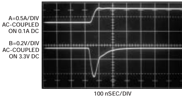
Figure 21 An excessively lossy 10\text{-}\mu\text{F} C_{\text{OUT}} allows a 400-mV excursion—four times Figure 18's amount. The time skewing between the traces derives from probe mismatch.
