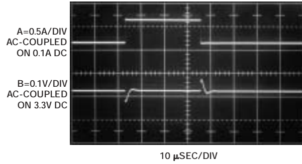
Figure 22 Replacing C_{OUT} with a low-loss, 33- \mu F unit yields a 40% smaller output-response transient than that of Figure 17.
