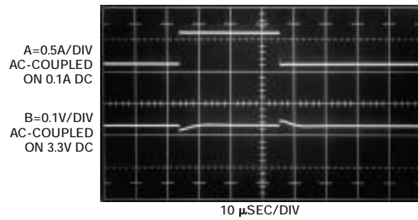
Figure 23 A low-loss, 330- \mu F capacitor keeps output-response transients to less than 20 mV—four times lower than Figure 17's 10- \mu F capacitor.
