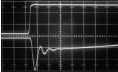
Figure 25 Faster rise-time current step (Trace A) increases response-decay peak (Trace B) to 140 mV, indicating increased regulation loss versus frequency.
