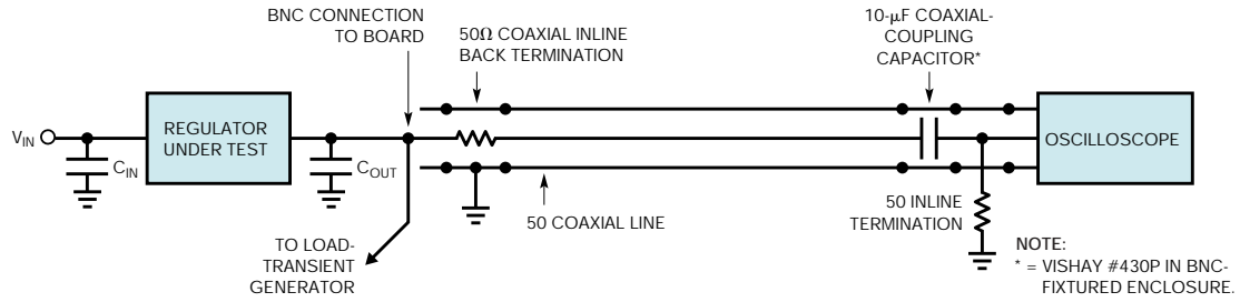
Figure A A coaxial-load-transient voltage-measurement path promotes observed signal fidelity. You can remove the 50Ω back termination with minimal impact on the 25-MHz signal path's integrity.
