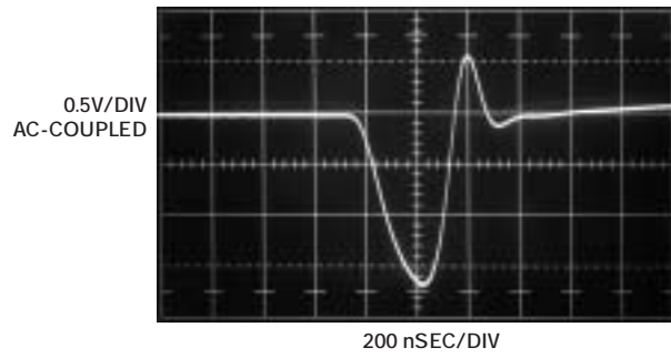
Figure B Observing a typical high-speed transient through Figure A's measurement path presents a clean and well-defined signal.
