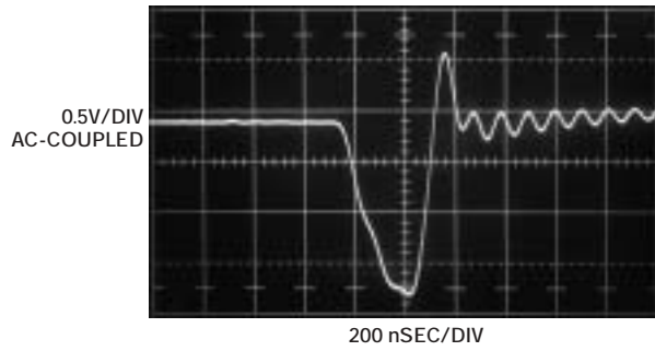
Figure C Measuring Figure B's transient without the 50\Omega oscilloscope's termination shows results in waveform distortion and postevent ringing.
