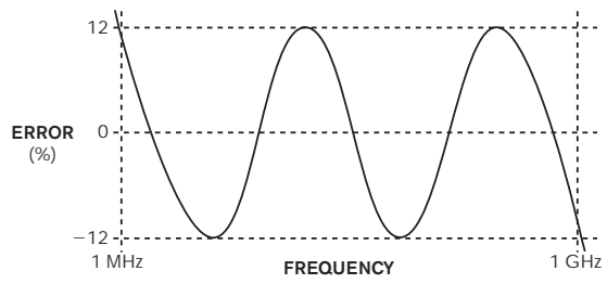
Figure 6 The Spice model in Figure 5 agrees with Table 1 within 12% over a 1000-to-1 frequency range.
