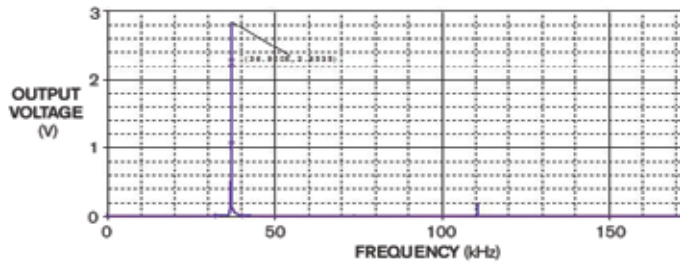
Figure 4 The oscillator's output spectrum shows only a slight amount of third-harmonic output.
