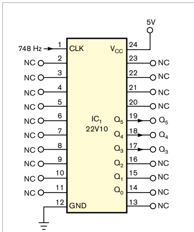
Figure 1 An external 748-Hz clock source drives this PLD-based, three-phase sine-wave generator.
