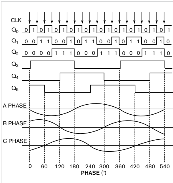
Figure 3 The timing diagram shows the relationship between the clock and the three-phase outputs.
