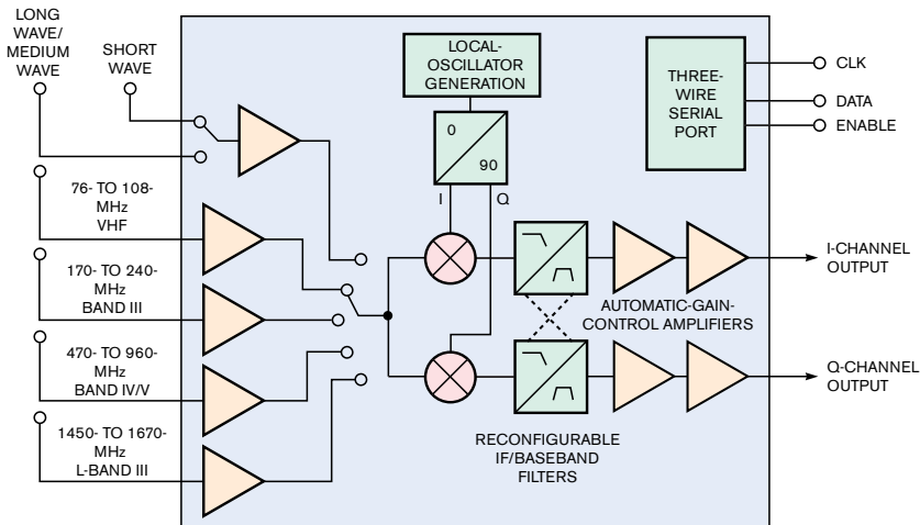
The MS1001 RF-tuner IC covers multiple broadcast standards at 100 kHz to 1.9 GHz.
