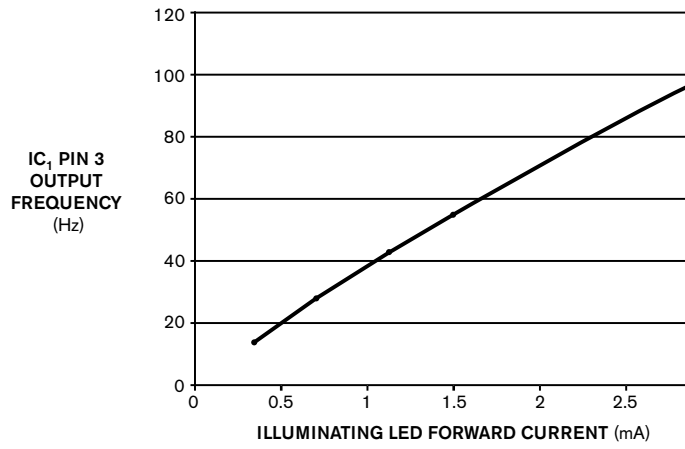
Figure 4 The frequency of the circuit's square-wave output exhibits good linearity versus light level for identical sensor and source LEDs.
