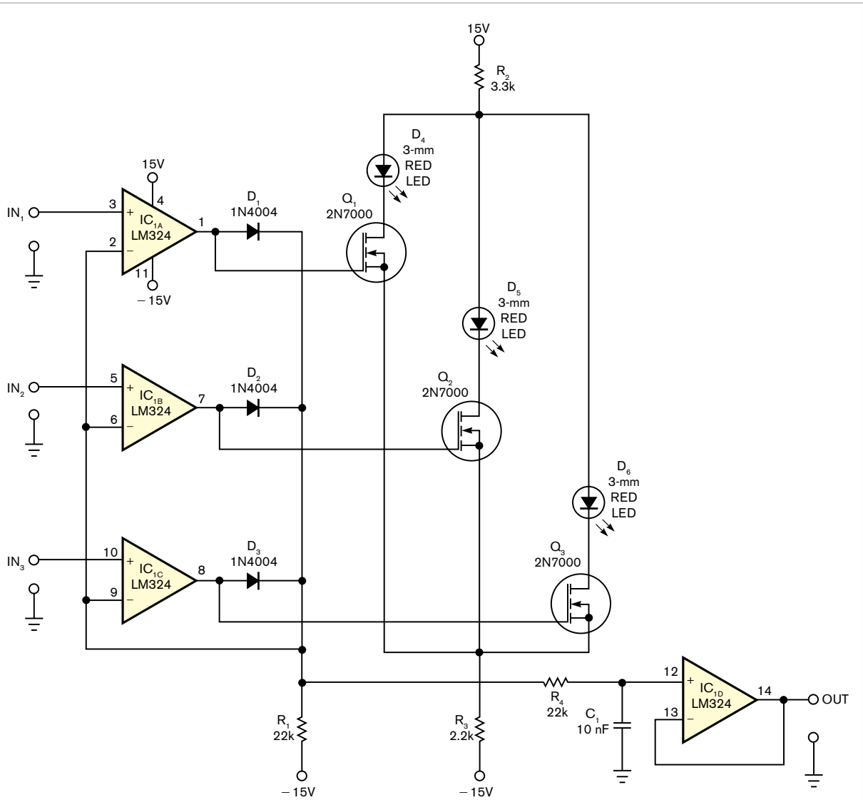
Figure 1 This circuit's output voltage tracks and indicates the highest of three input voltages and can drive an external strip-chart recorder or alarm comparator.
