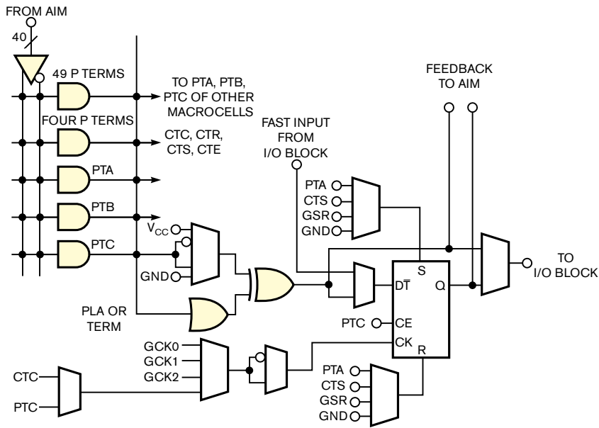
Figure B CoolRunner-II macrocells accommodate as many as 56 inputs.
