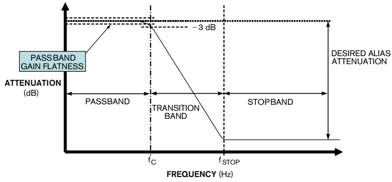
Figure 2 Ideal lowpass antialiasing filters should have a steep transition band, excellent gain flatness, and low distortion in the passband.
