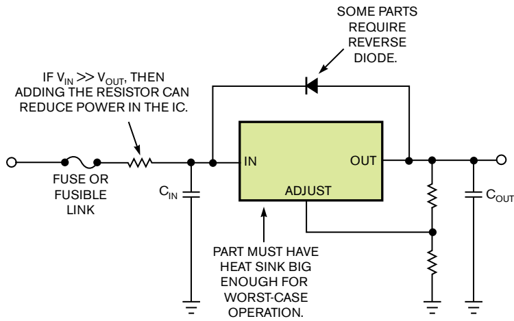
Figure 1 Linear supply problems are heat, capacitor shorting, and damage to the part when reverse currents flow inside the IC.
