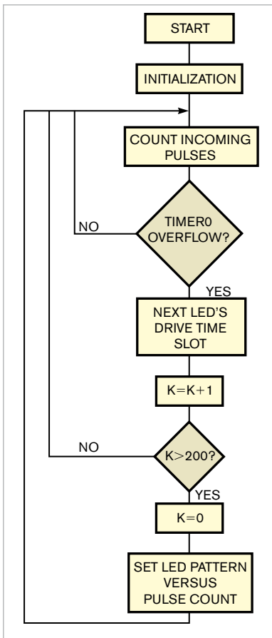
Figure 3. This flow chart shows the LED-driver software routine. (See the listings at www.edn.com/061215di1 for the complete tachometer routine.)
