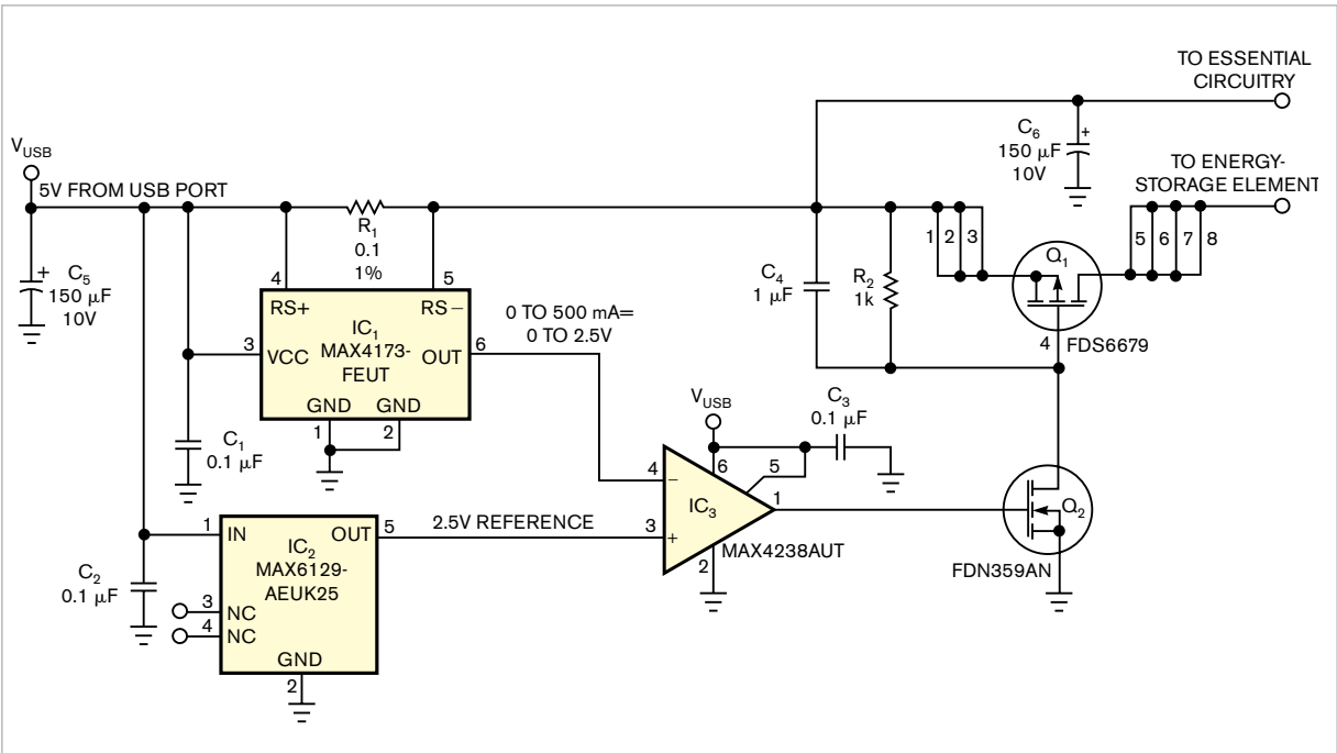
Figure 2 This circuit continuously monitors the total current drawn from the USB port and dynamically adjusts the storage-element current to avoid exceeding the port's maximum output capability.
