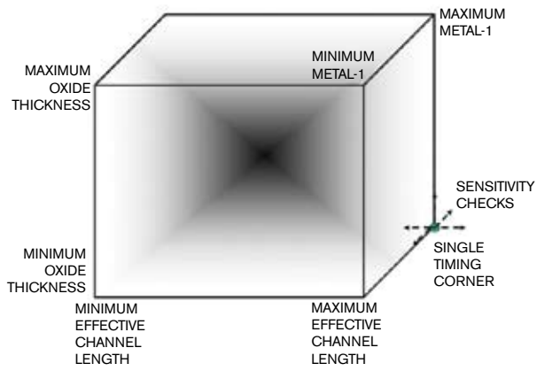
Figure A IBM's statistical timing approach starts from one process point and computes sensitivities, rather than performing analysis at all possible corners.
