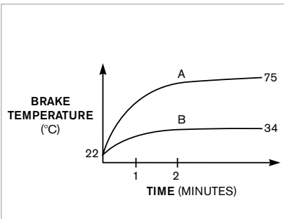
Figure 1 Under continuous operation with 24V applied, the brake's temperature stabilizes at 75°C, or 53°C above ambient temperature (Curve A). Applying a 24V actuation pulse for a few seconds and then applying a 12V holding voltage stabilizes the brake at 34°C, or only 12°C above ambient temperature (Curve B).
