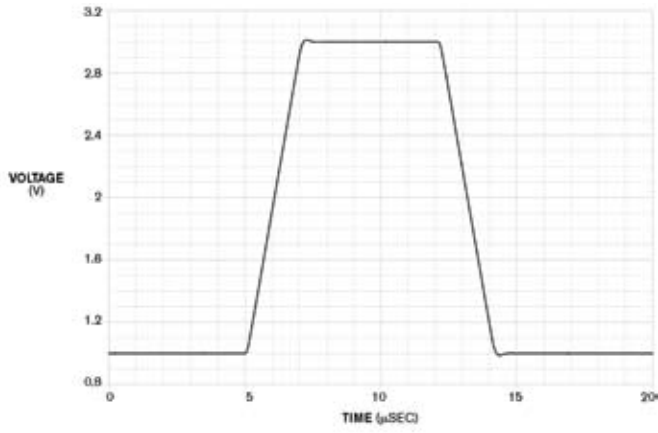
Figure 4 In this plot of the macromodel-voltage-follower pulse response, the slew rate is 1 MV/sec.
