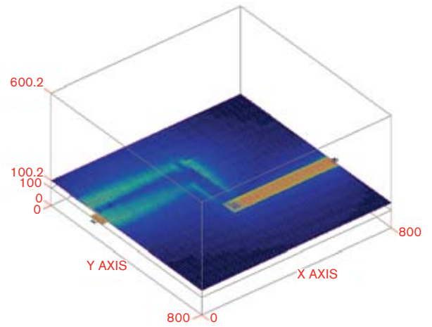
Figure 1 A user can directly model circuit traces, or the layout package can feed back the physical configuration (a). The field solver uses this input (b) to calculate the fields, voltages, and currents (courtesy Applied Wave Research).
