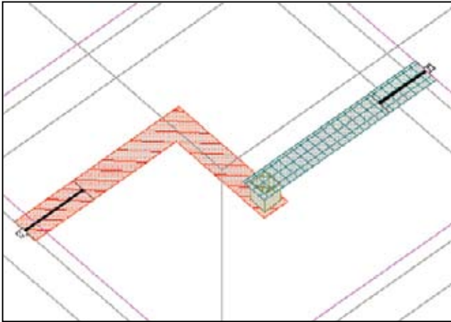
Figure 1 A user can directly model circuit traces, or the layout package can feed back the physical configuration (a). The field solver uses this input (b) to calculate the fields, voltages, and currents (courtesy Applied Wave Research).
