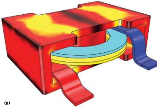
Figure 3 Field solvers can provide results for intractable problems involving nonlinear magnetics (a) as well as complex 3-D spiral inductors (b) (courtesy Comsol).
