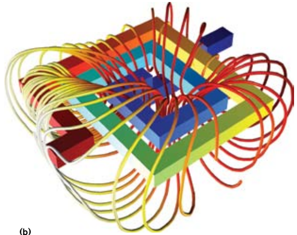
Figure 3 Field solvers can provide results for intractable problems involving nonlinear magnetics (a) as well as complex 3-D spiral inductors (b) (courtesy Comsol).
