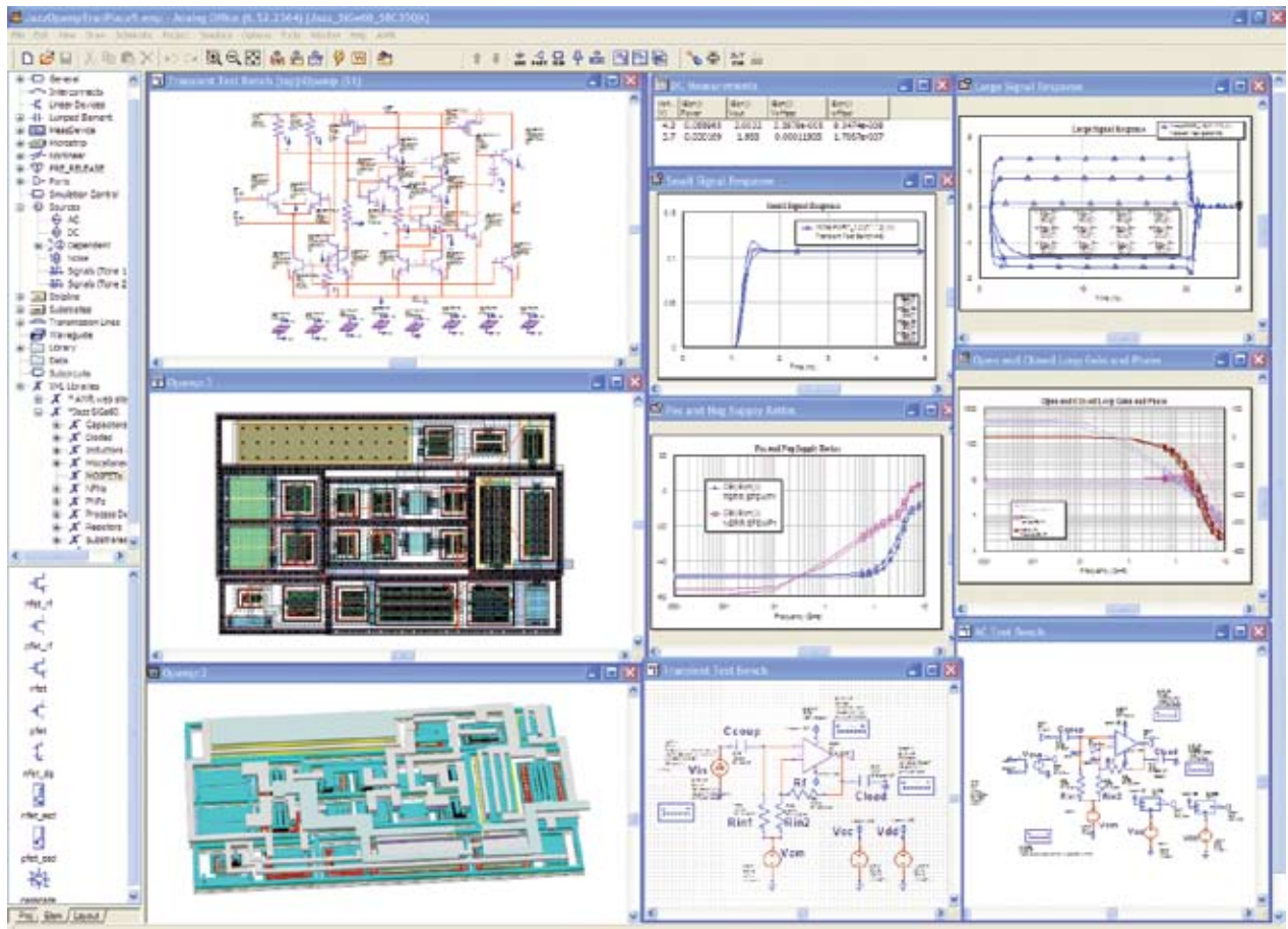
Figure 4 A full-blown design environment allows schematic entry, time- and frequency-domain simulation, layout, and field solvers for signal-integrity and RF design (courtesy Applied Wave Research).
