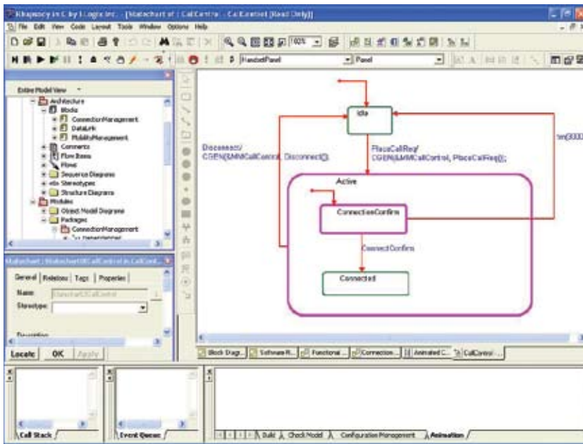
Figure 1 The recently introduced Version 7.0 Rhapsody from Telelogic generates C, C++, or Java code directly from a standard UML model.
