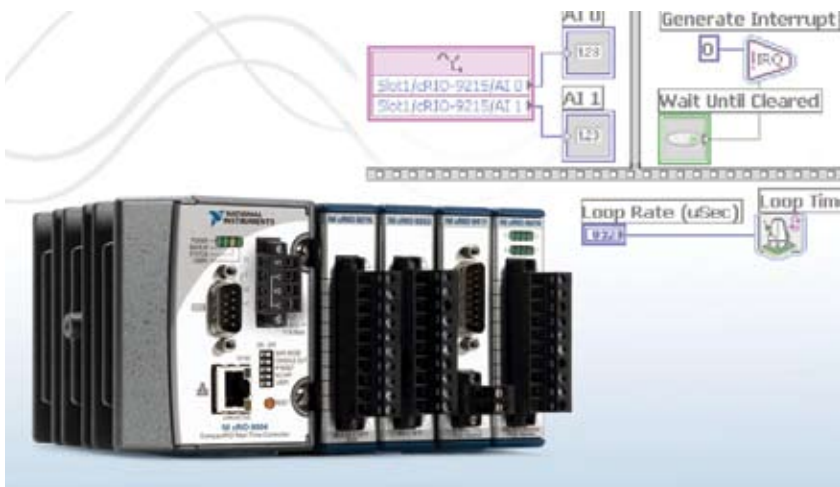
Figure 5 The CompactRIO system from National Instruments defines custom hardware circuitry using a reconfigurable FPGA and LabView graphical-development tools.
