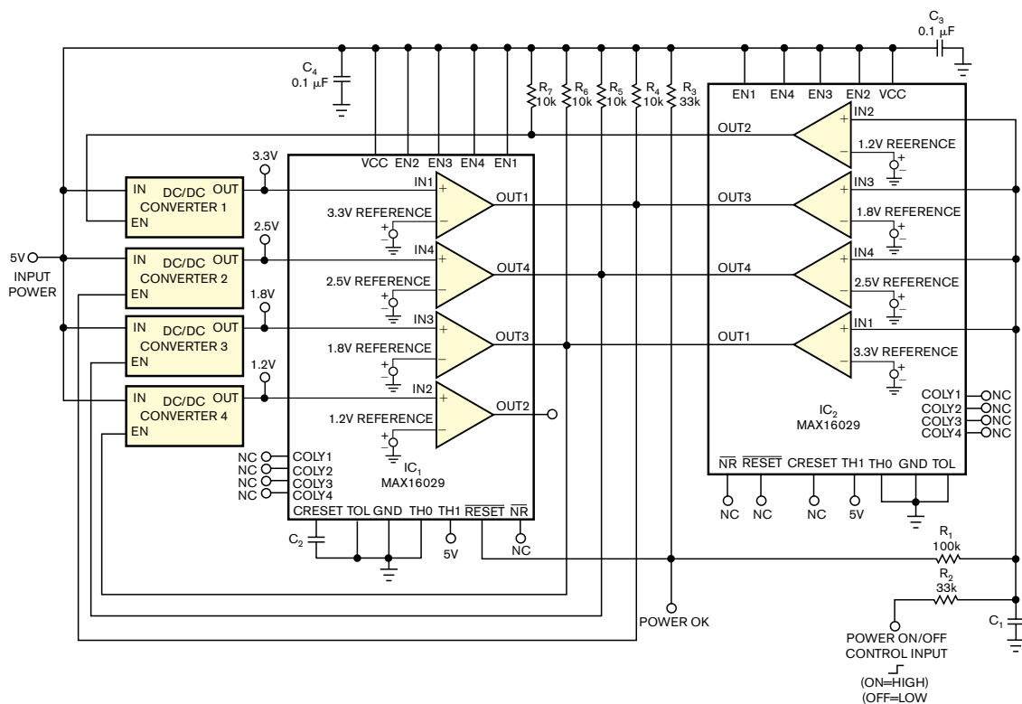
Figure 1 Comprising a pair of inexpensive ICs, this circuit applies four supply voltages in a specified order at power-up and then removes them in reverse order at power-down.
