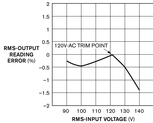
Figure 3 The line monitor has 0.5% accuracy from 90 to 130V ac, degrading to 1.4% accuracy at 140V ac. Almost all the error is due to transformer parasitic losses.
