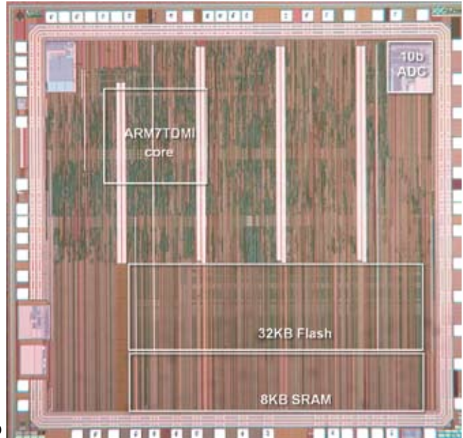
(a) (b) Figure 1 These die shots of a 16-bit (a, courtesy Texas Instruments) and a 32-bit (b, courtesy NXP) processor illustrate the relative silicon area of the processor core and on-chip memory (not to scale with each other).
