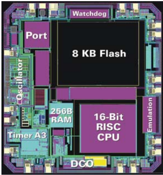
(a) (b) Figure 1 These die shots of a 16-bit (a, courtesy Texas Instruments) and a 32-bit (b, courtesy NXP) processor illustrate the relative silicon area of the processor core and on-chip memory (not to scale with each other).
