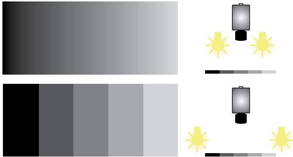
Figure A Incorrect lighting in a machine-vision system can eliminate the visibility of the features upon which the system bases control (courtesy Edmund Optics).
