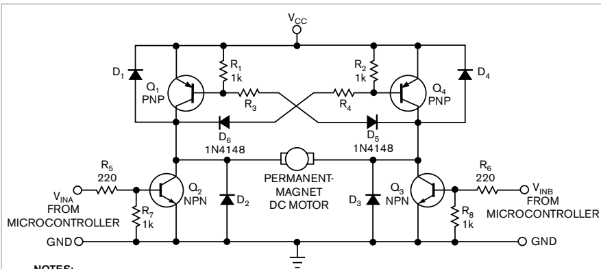
Figure 2 This improved H-bridge-driver circuit uses transistors in complementary pairs and requires only two low-level control signals.
