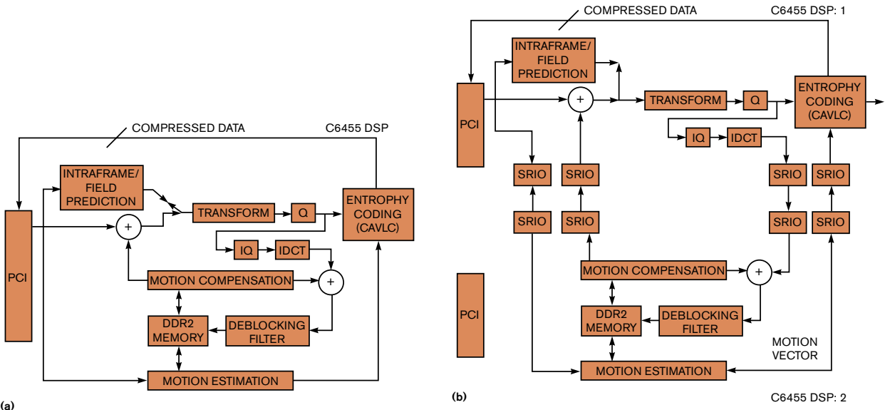
Figure 4 SD (a) and HD (b) encoding require, respectively, one and two 1-GHz DSPs.
