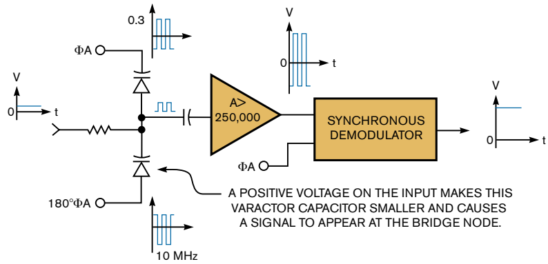
Figure C A varactor-bridge amplifier has the input voltage unbalance the equal varactor capacitors, which creates an ac voltage. The process then amplifies that voltage and demodulates it back to dc.
