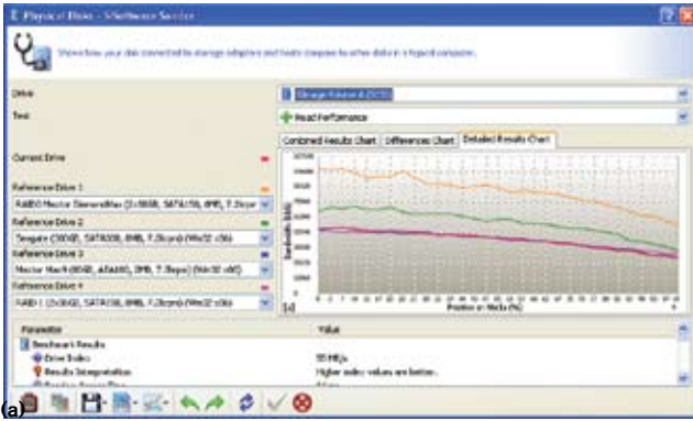
Figure 3 Single-drive- (a) and multidrive-concatenated (b) configurations both reveal varying data-transfer rates across a hard drive's platter.
